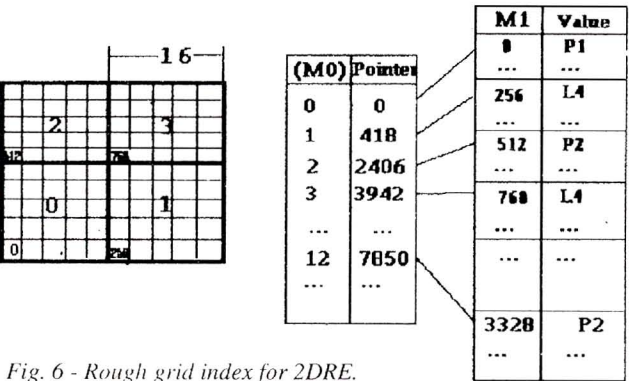
Fig. 6 - Rough grid index for 2DRE.
