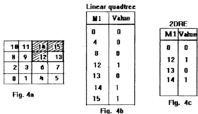
Fig. 4 - Linear quadtree and 2DRE.
