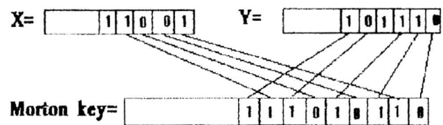
Fig. 3 - Generation of Morton key.
