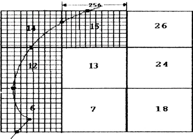
Fig. 5 - Morton keys of basic grids and fine-divided grids.
