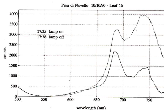
Fig. 14 - Remote night-time fluorescence recordings of green beech leaves. Spectra were recorded in darkness and during light exposure with a flashlight. a) Recordings with the Lund system (lexc=355 nm). b) Recordings with the CNR-IROE system (lexc=480 nm).
